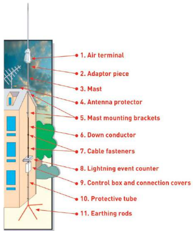
Lightning rod with feeder device [Source: CIRPROTEC]
